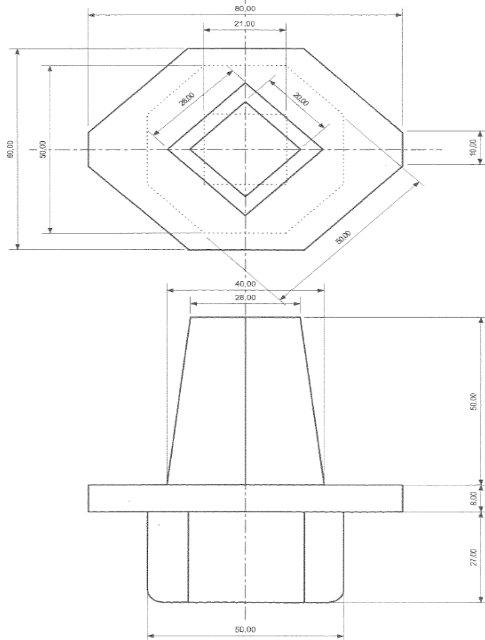
Dimensions of the operating cap Type B
